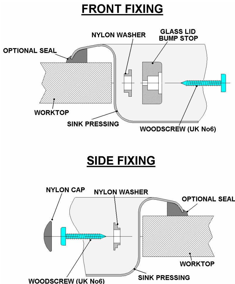
Fig. 1. Fixing Details
